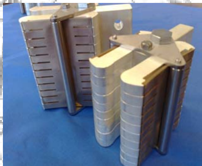
High Voltage Breaker Contacts
